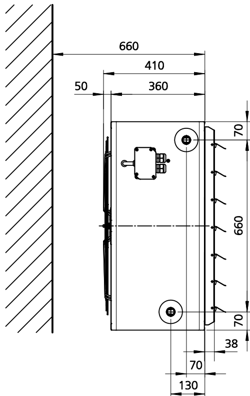
Wandmontage
